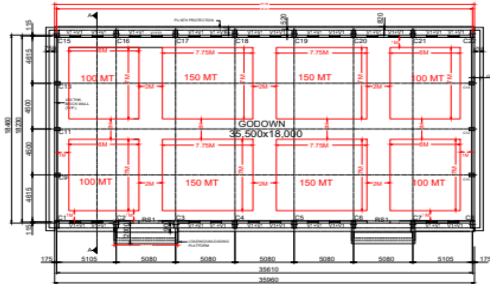
PLAN SCALE - 1:100
